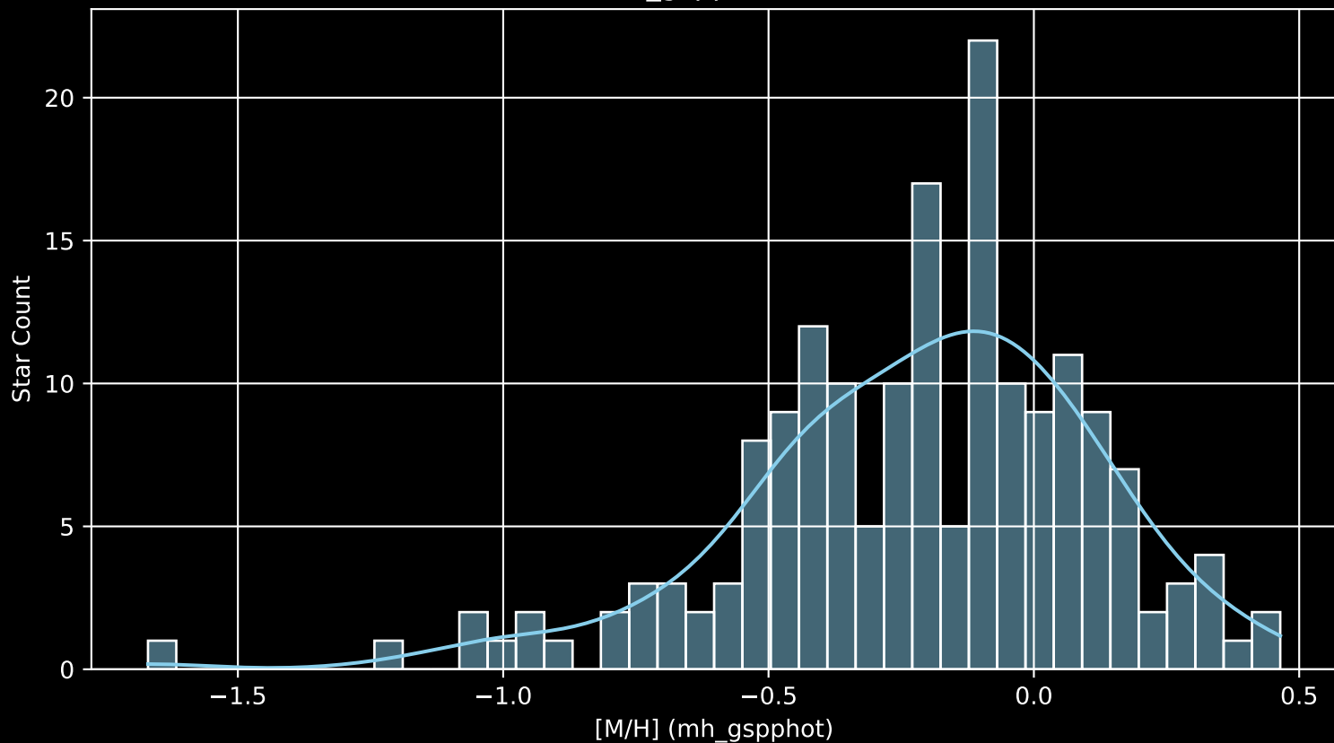
APOGEE DR17 Field: [INTCL_N6229_MGA [M/H] (mh_gspphot) (n= 177)
