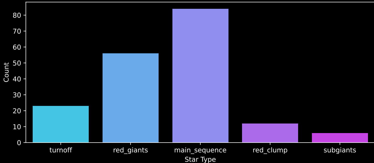
APOGEE DR17 Field: [INTCL_N6229_MGA] Count plot of Star Type
