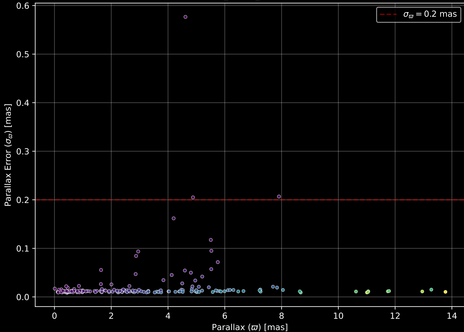
APOGEE DR17 Field: [INTCL_N6229_MGA] Parallax Quality (n= 181)
