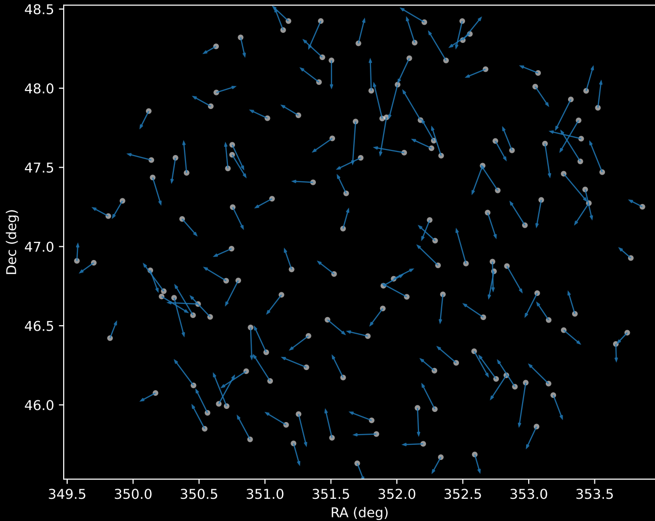
APOGEE DR17 Cluster 0 Proper Motion Vectors (n=144)
