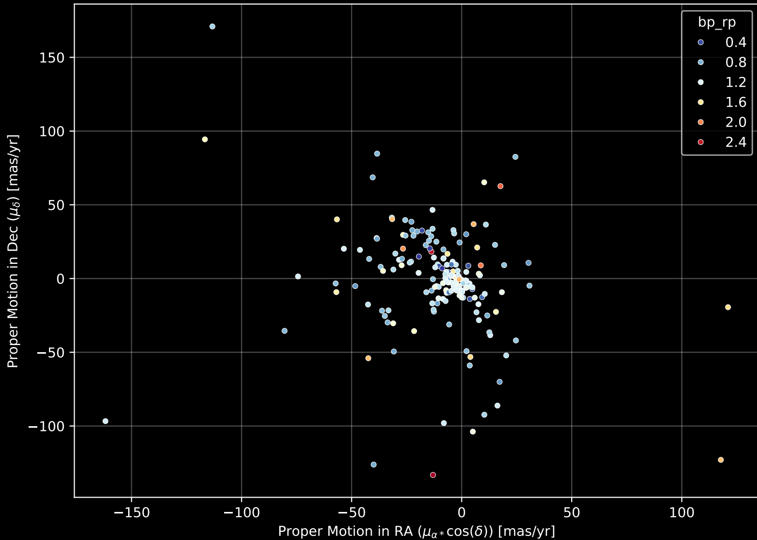
APOGEE DR17 Field: [INTCL_N6229_MGA] Proper Motion Diagram (n= 181)
