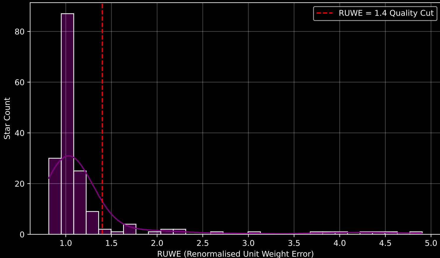
GAPOGEE DR17 Field [INTCL_N6229_MGA] RUWE Distribution (n= 172)
